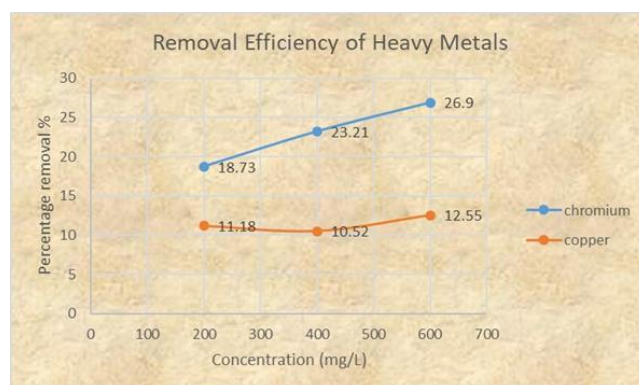
Figure 3: Removal Efficiency of Heavy Metals
