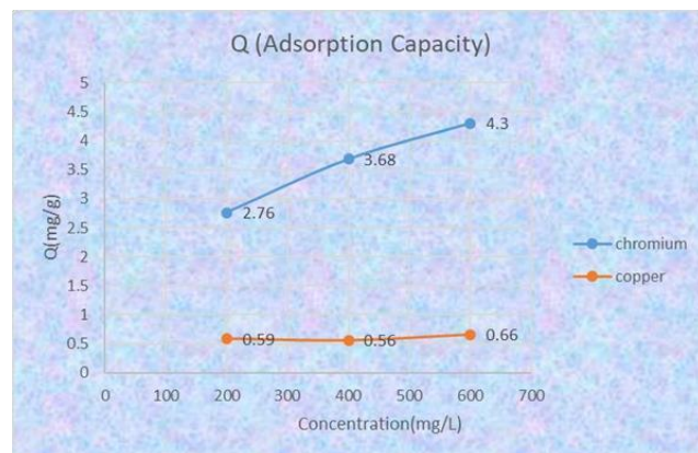
Figure 2: Adsorption capacity for the heavy metals
